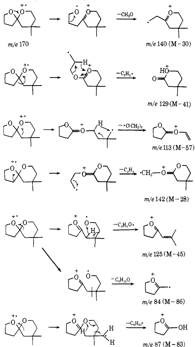
Chart II. Mass Spectral Fragmentation of 9,9-Dimethyl-1,6-dioxaspiro[4.5]decane ( 8 )
