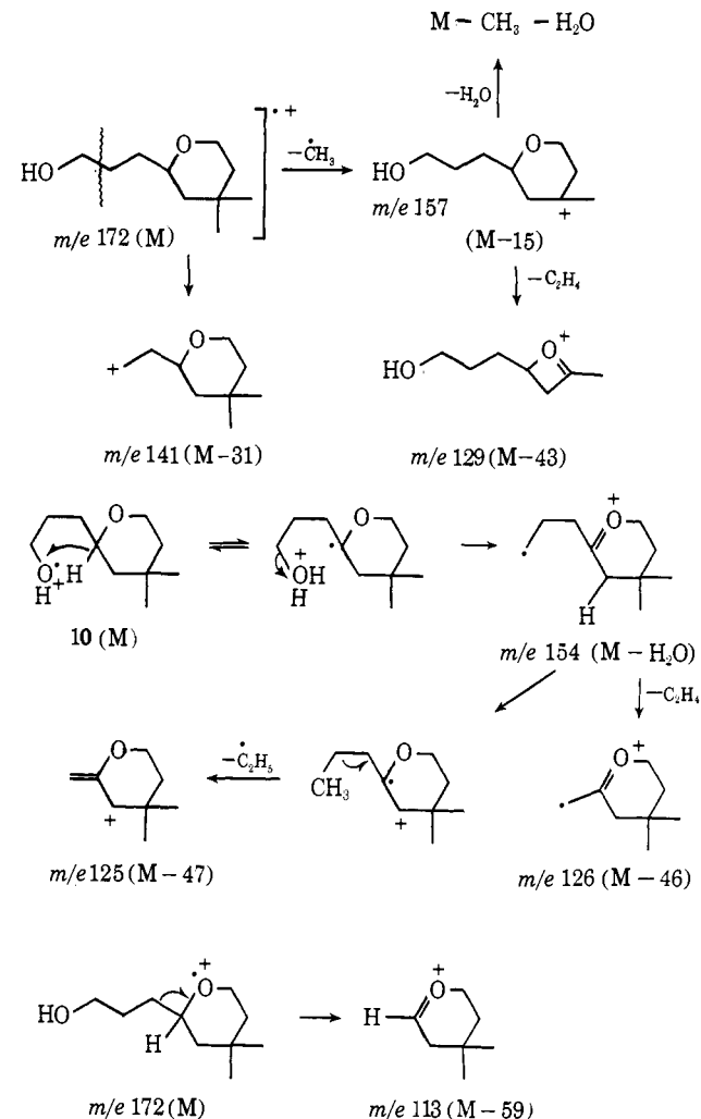
Chart III. Mass Spectral Fragmentation of 2-(3'-Hydroxypropyl)-4,4-dimethyltetrahydropyran ( 9a )
